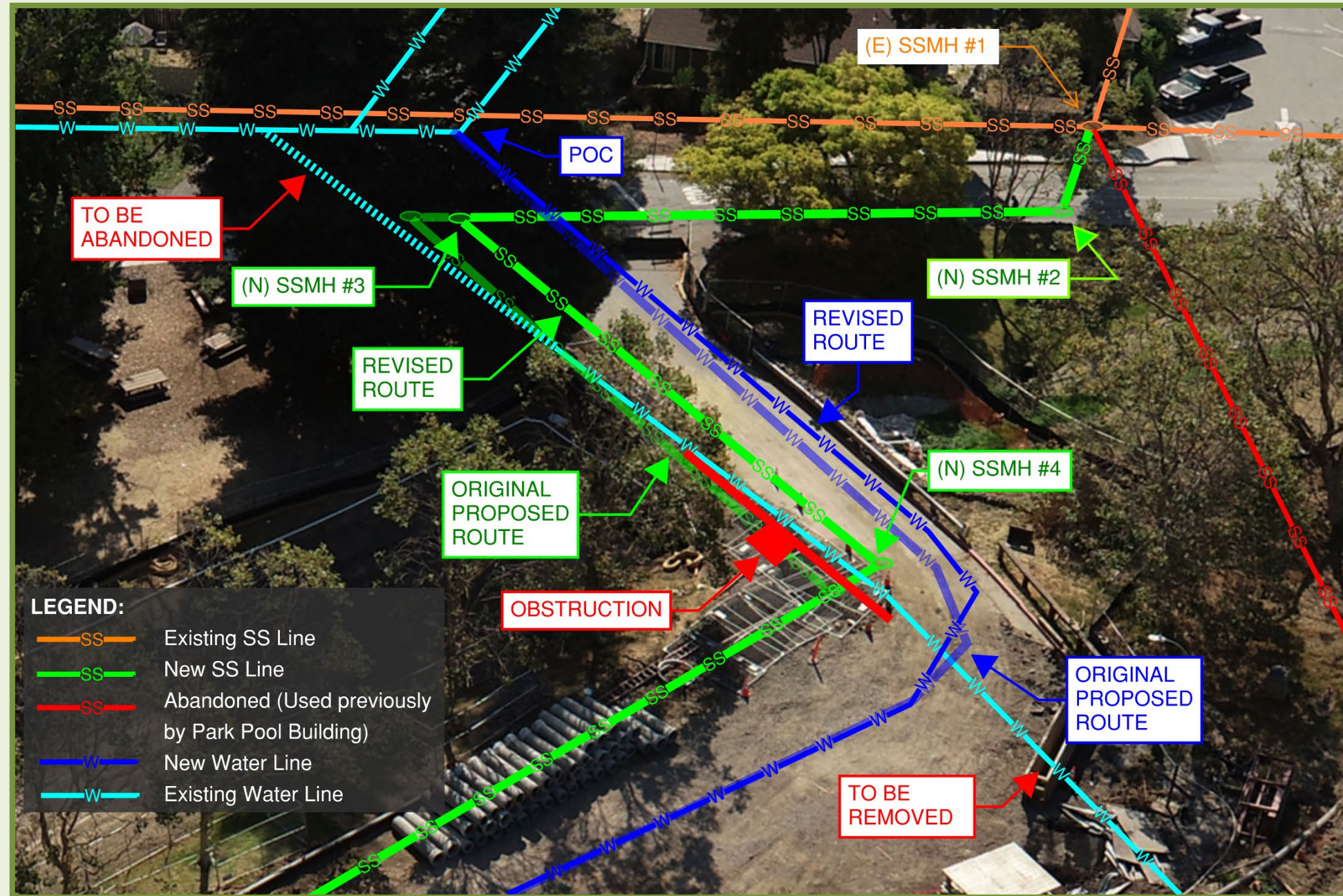
UTILITY UPDATE: SEWER
