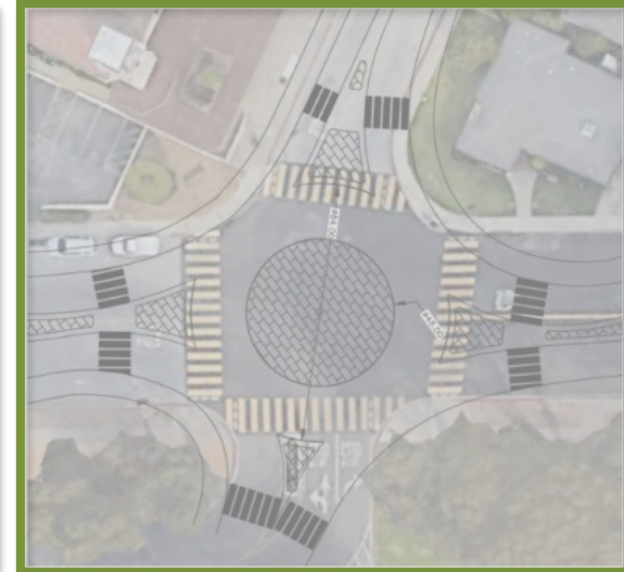
Single-lane Roundabout (RA-1)
